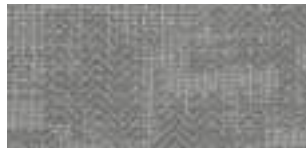
Boulder 1012485
